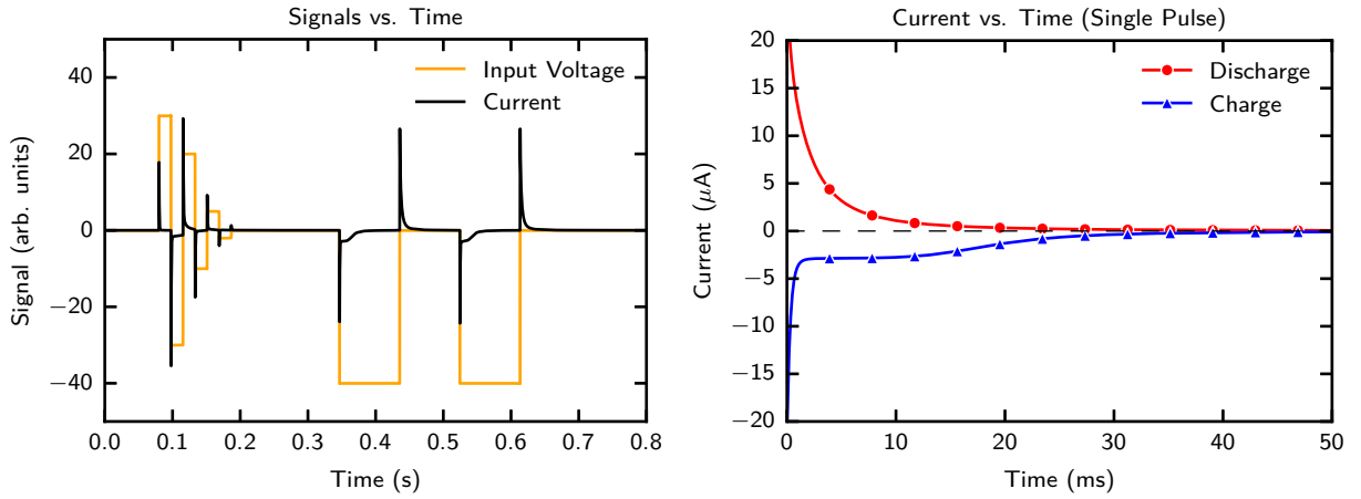
Figure 4.10: DLTS excitation waveform and representative single-pulse transient response. The left panel shows the applied voltage pulses together with the corresponding current response. The right panel compares the charge and discharge transients after one pulse, showing a fast initial response followed by a slower relaxation towards the baseline.
