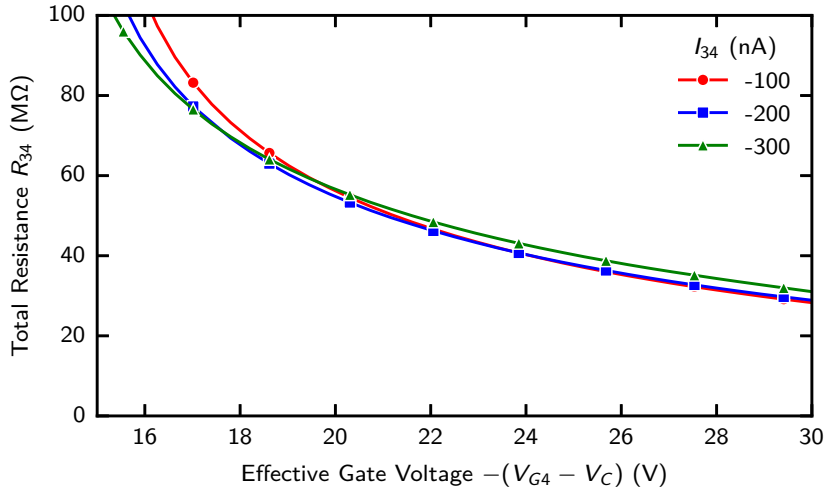
Figure 4.8: Total resistance R_{34} = |V_{34}/I_{34}| versus effective gate voltage V_{\text{eff}} = -(V_{G4} - V_C) for three imposed currents. The resistance decreases with increasing V_{\text{eff}} , and the three current series nearly overlap, with a small upward shift for the -300 nA series at larger V_{\text{eff}} .
