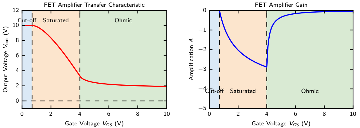
Figure 2.12: FET amplifier transfer characteristic and small-signal gain. The left panel shows the static output voltage as a function of gate bias. The local slope of this curve determines the voltage gain shown on the right. The gain is negative in the inverting common-source configuration and is largest in magnitude within the transition region between cut-off and strongly ohmic operation.
