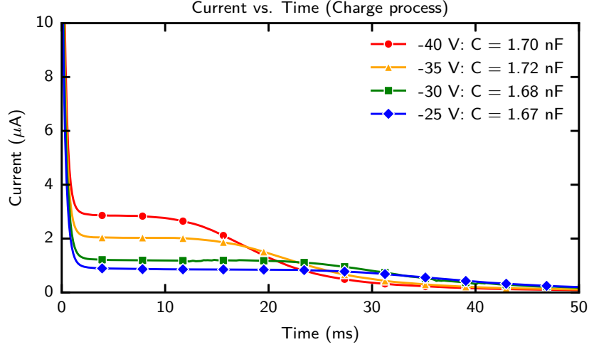
Figure 4.11: Full DLTS transient trace recorded during the charge process for different applied bias levels. The current relaxes after the voltage step and approaches a low background value. The effective capacitance is determined from C_{\text{eff}} = Q/V_0 , with Q obtained by integrating the transient current. The extracted values remain close to 1.7 nF, indicating that the dominant fast contribution is capacitive, while the slower tail is associated with trap-related relaxation.
