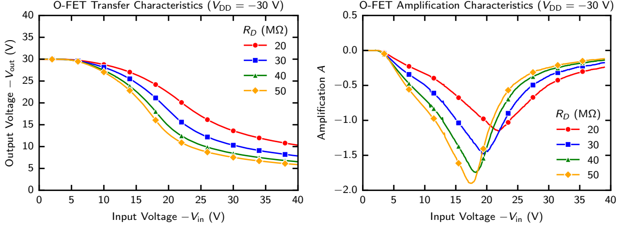
Figure 4.13: Transfer curve and amplification characteristic at V_{DD} = -30 V for different drain-load resistances R_D . The transfer plot identifies the input-voltage range where the output voltage changes most strongly, while the amplification plot shows the corresponding small-signal voltage gain. Larger R_D values increase the maximum gain but also narrow the useful operating range.
