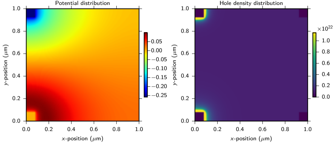
Figure 2.14: Calculated potential and hole-density distributions in the lateral van der Pauw structure. The potential map is obtained by iteratively solving Poisson’s equation on the two-dimensional grid with fixed contact potentials and insulating outer boundaries. The hole-density map is then calculated from the Boltzmann approximation and shows hole accumulation near the current-carrying contacts.
