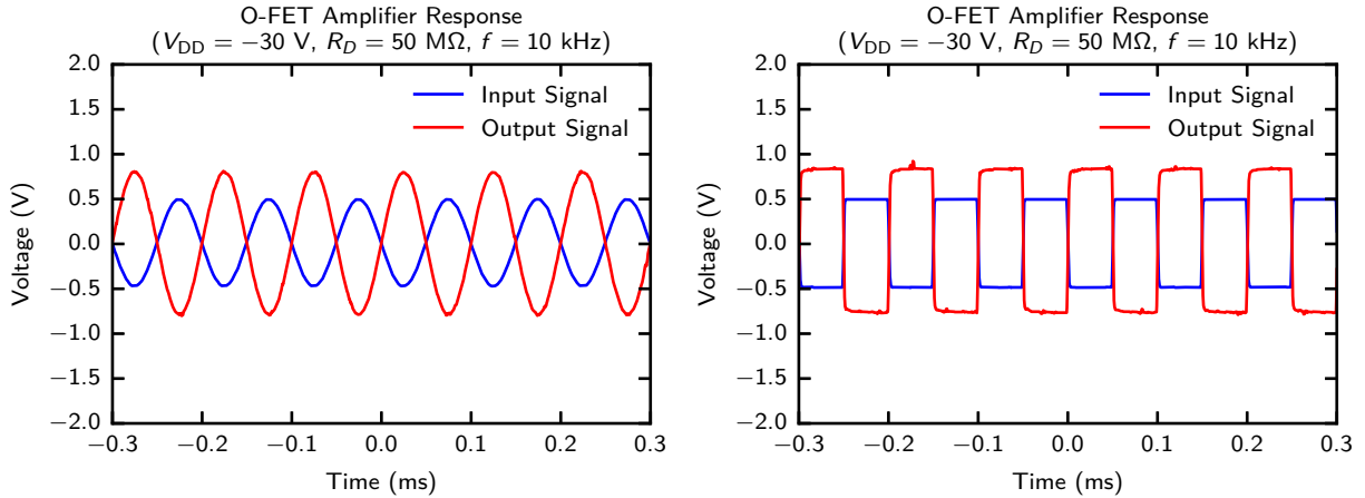
Figure 4.14: Dynamic response of the thin-film amplifier at V_{DD} = -30 V, R_D = 50 M \Omega , V_{G,Q} = -18 V, and f = 10 kHz. The sinusoidal measurement demonstrates inverted voltage amplification, while the square-wave measurement shows the finite rise and fall times caused by the large circuit resistance, device capacitance, and trap-related relaxation.
