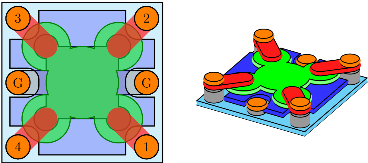
Figure 3.2: Schematic representation of the assembled thin film structure. The left panel shows the top-view contact layout, while the right panel shows the corresponding 3D layer structure.
