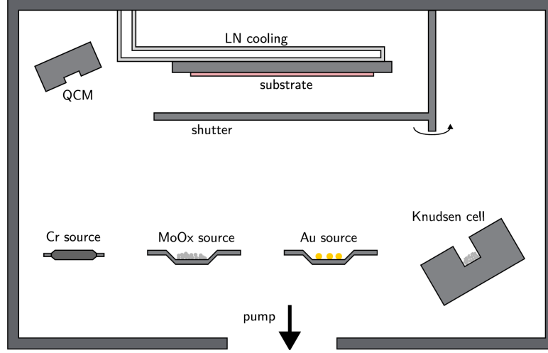
Figure 3.3: Schematic of the physical vapor deposition (PVD) system. Figure from Ref. [22].
