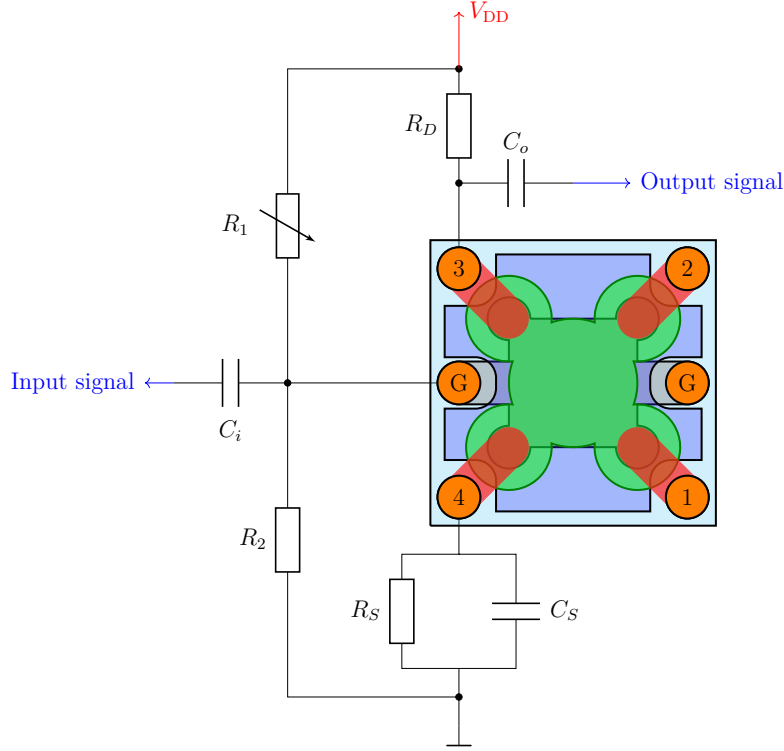
Figure 4.12: Circuit used to analyse the amplification properties of the gated thin-film device. The input signal is capacitively coupled to the gate through C_i = 1 \text{ nF} , while the gate operating point is set by the bias divider with R_2 = 100 \text{ k}\Omega and variable R_1 . The drain is biased through R_D at V_{DD} = -30 \text{ V} , with R_D varied from 20 \text{ M}\Omega to 50 \text{ M}\Omega . The output signal is measured at the drain contact through C_o = 1 \text{ nF} . The source branch contains R_S and the bypass capacitor C_S = 1 \text{ nF} , which set the source bias and influence the small-signal response.
