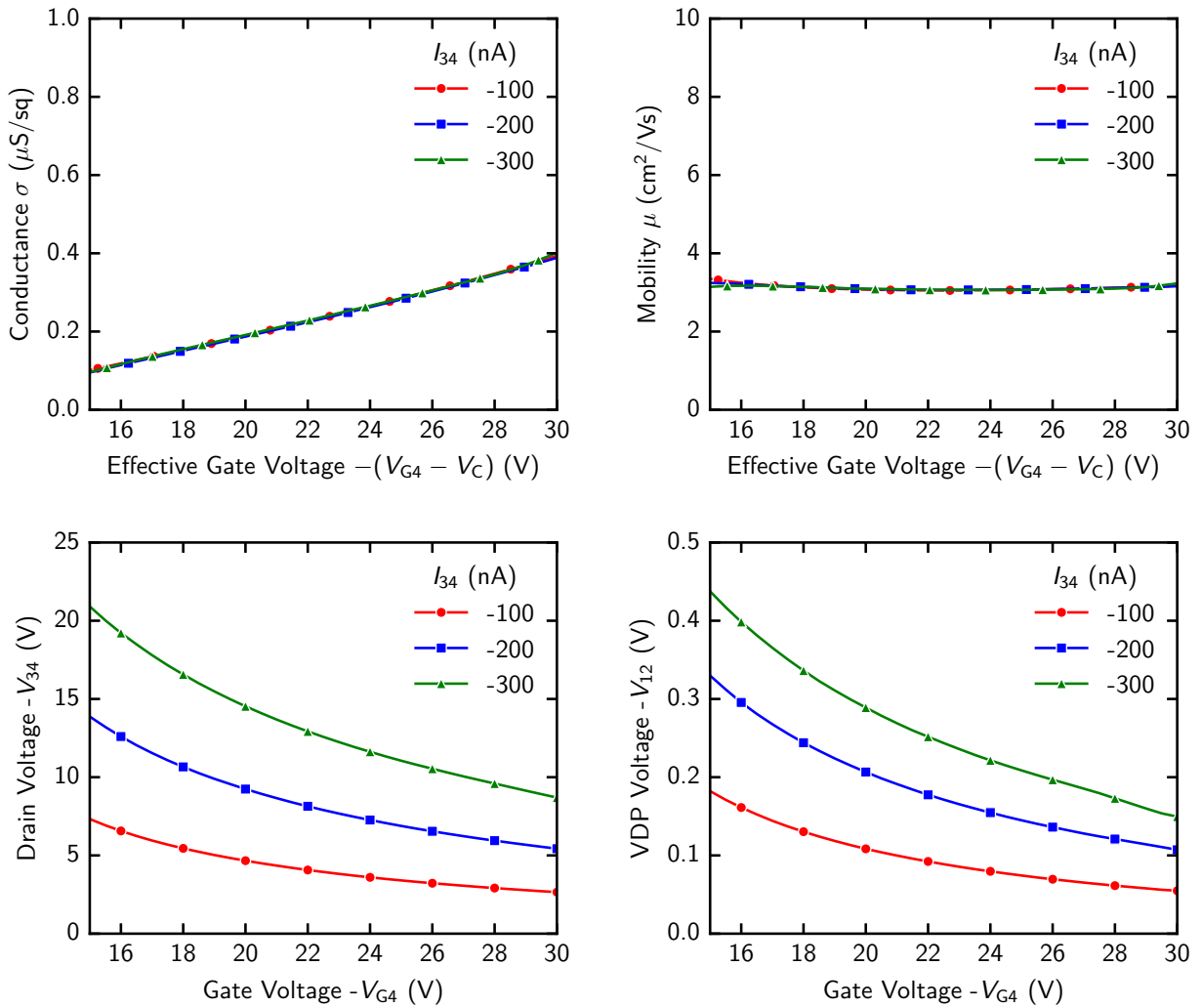
Figure 4.7: Gated van der Pauw extraction for I_{34} = -100 \text{ nA} , -200 \text{ nA} , and -300 \text{ nA} . The lower panels show the measured voltages, while the upper panels show the extracted sheet conductance \sigma and mobility versus effective gate voltage. The overlap of the three current series indicates linear-response behaviour and supports a current-independent mobility extraction.
