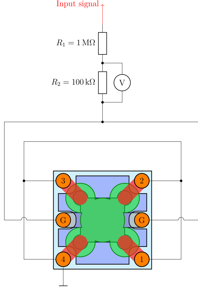
Figure 4.9: Circuit used for the deep-level transient spectroscopy (DLTS)-type measurements on the gated thin-film structure. The external excitation is applied through the resistive divider formed by R_1 = 1\text{ M}\Omega and R_2 = 100\text{ k}\Omega . The voltage across R_2 is monitored so that the transient response of the device can be followed after each bias perturbation.
