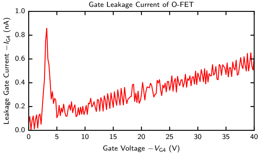
Figure 4.2: Gate-insulator leakage current of the gated thin-film structure, measured as -I_{G4} while sweeping the gate voltage -V_{G4} . The leakage current remains in the nanoampere range over the full voltage sweep, well below the 1\mu\text{A} limit. The isolated peak at low gate voltage is interpreted as a transient caused by a small dust particle, which is subsequently swept out by the applied electric field.
